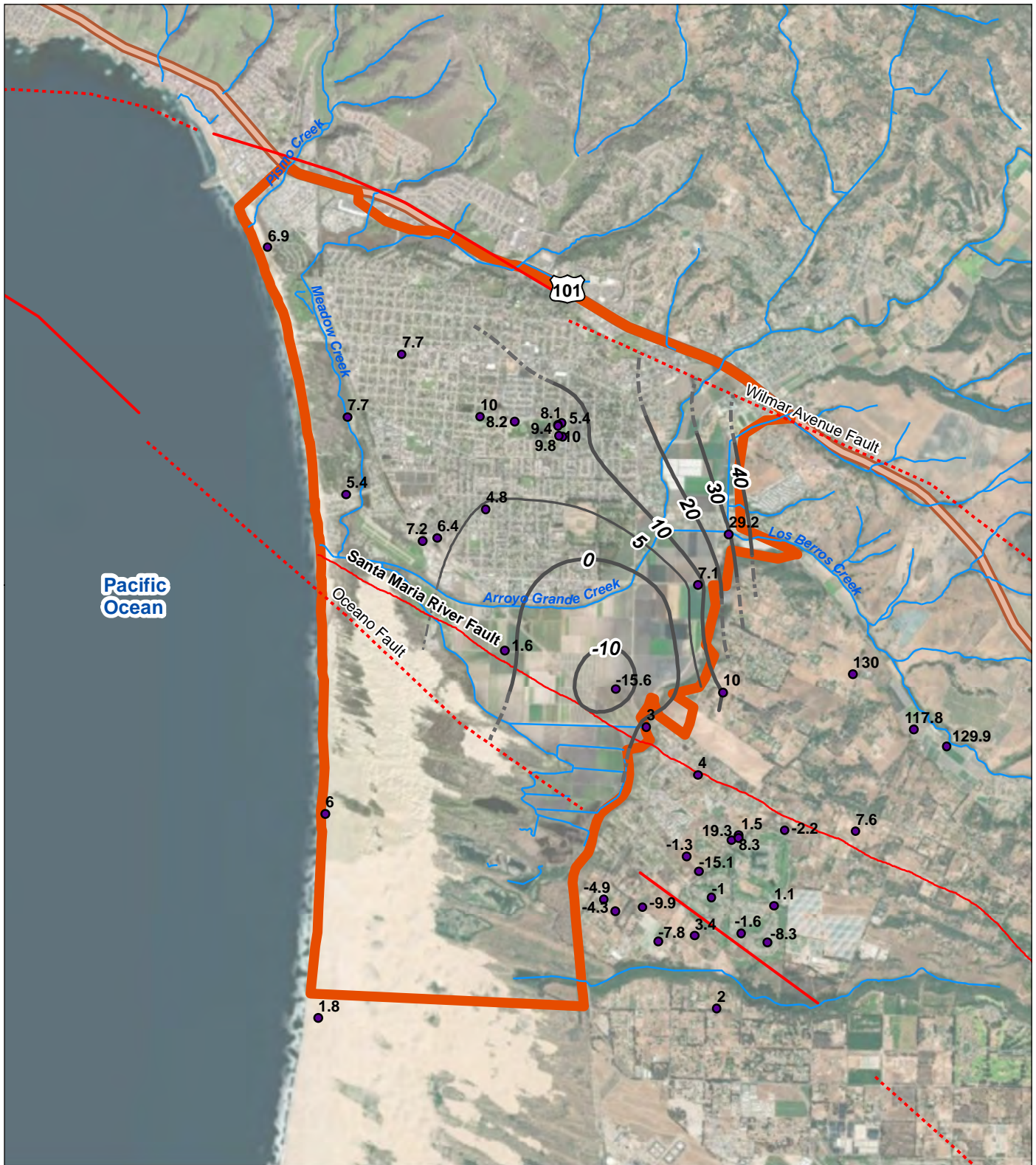
FIGURE 9 Groundwater Elevation Contours Fall 2018 Northern Cities Management Area San Luis Obispo County, California
