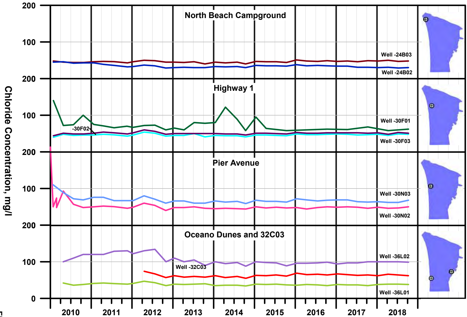
CHLORIDE CONCENTRATIONS IN MONITORING WELLS Northern Cities Management Area San Luis Obispo County, California
