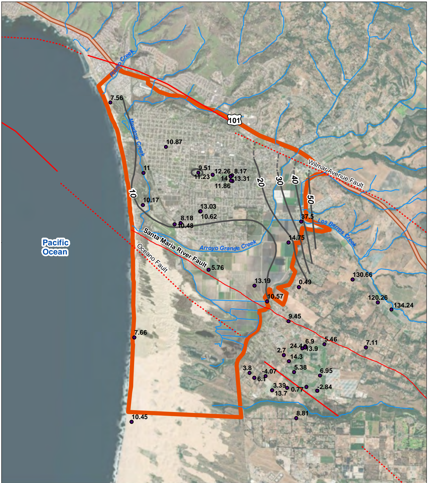
FIGURE 8 Groundwater Elevation Contours Spring 2018 Northern Cities Management Area San Luis Obispo County, California
